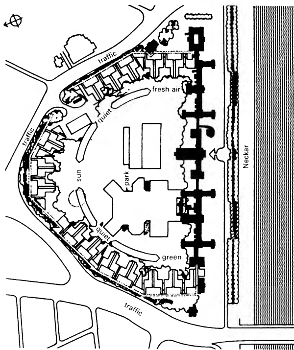
3 Rear of ward buildings along the periphery, blocking off traffic noise; all wards overlook the park
